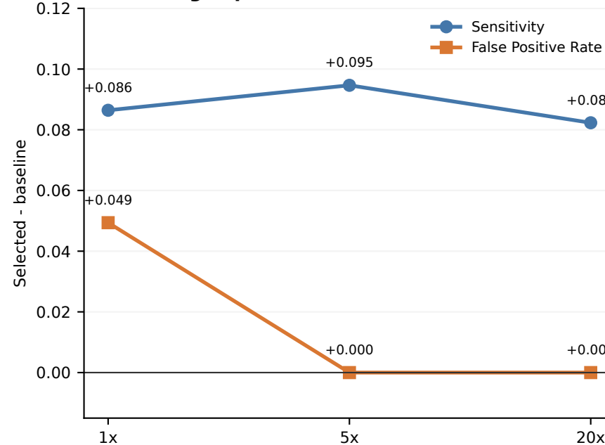
E Coverage-specific trade-off
