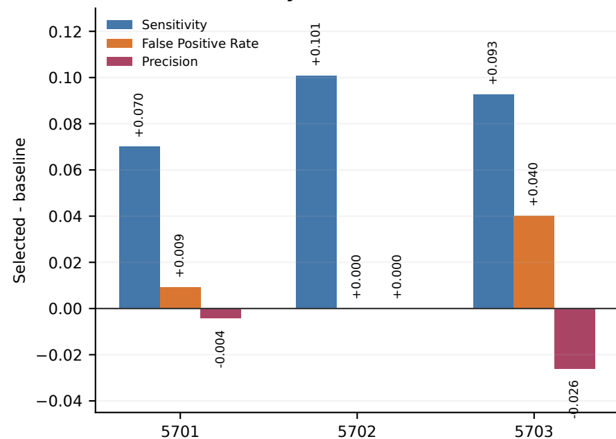
D Metric deltas by held-out seed
