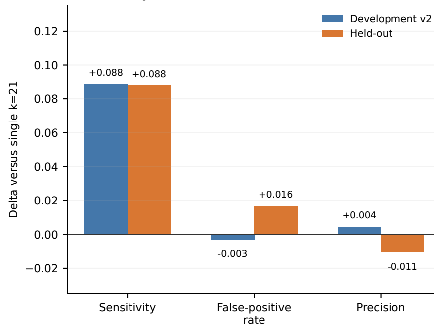
B Development-to-validation transfer
