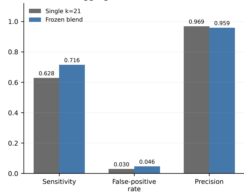
C Held-out aggregate metrics
