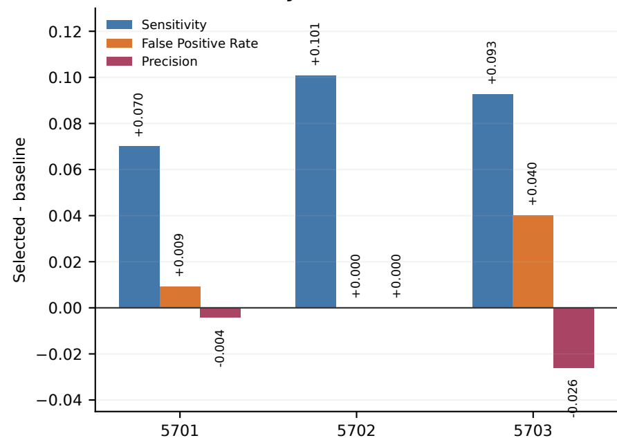
D Metric deltas by held-out seed
