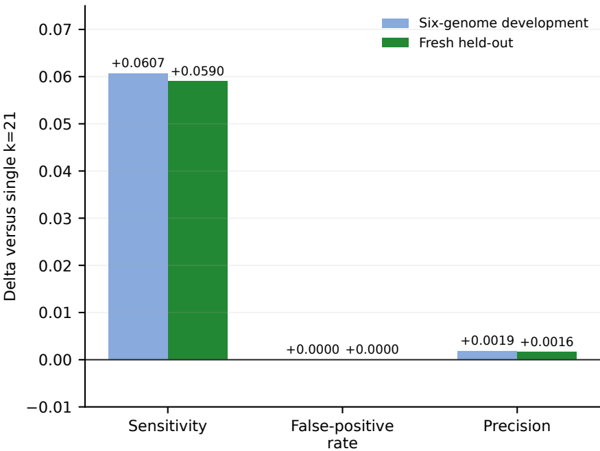
B Development and held-out deltas
