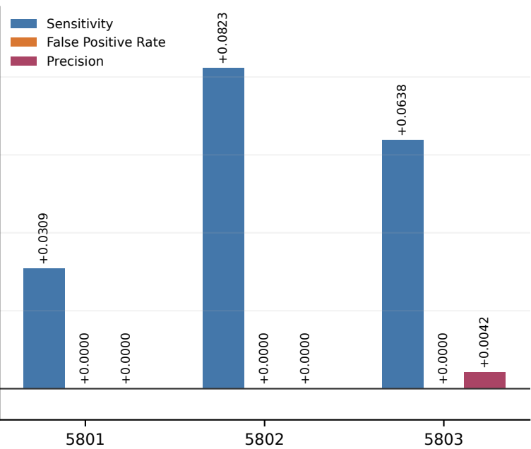
D Metric deltas by held-out seed
