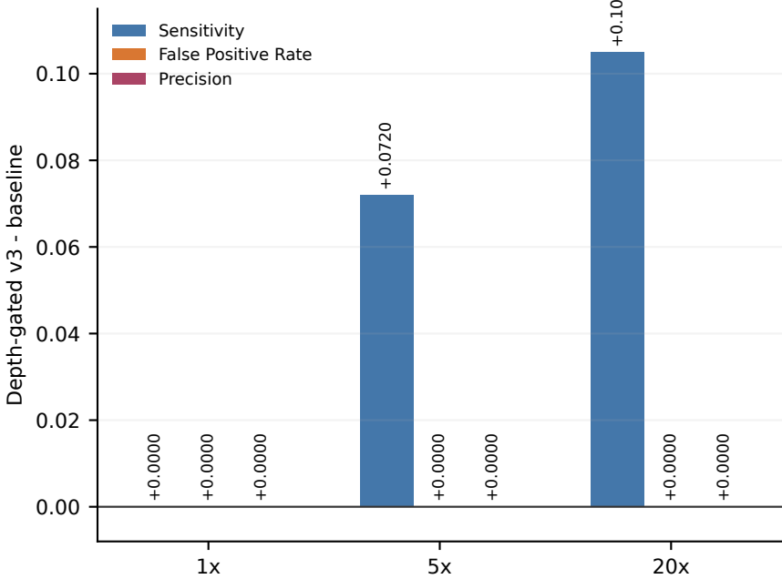
E Metric deltas by nominal coverage
