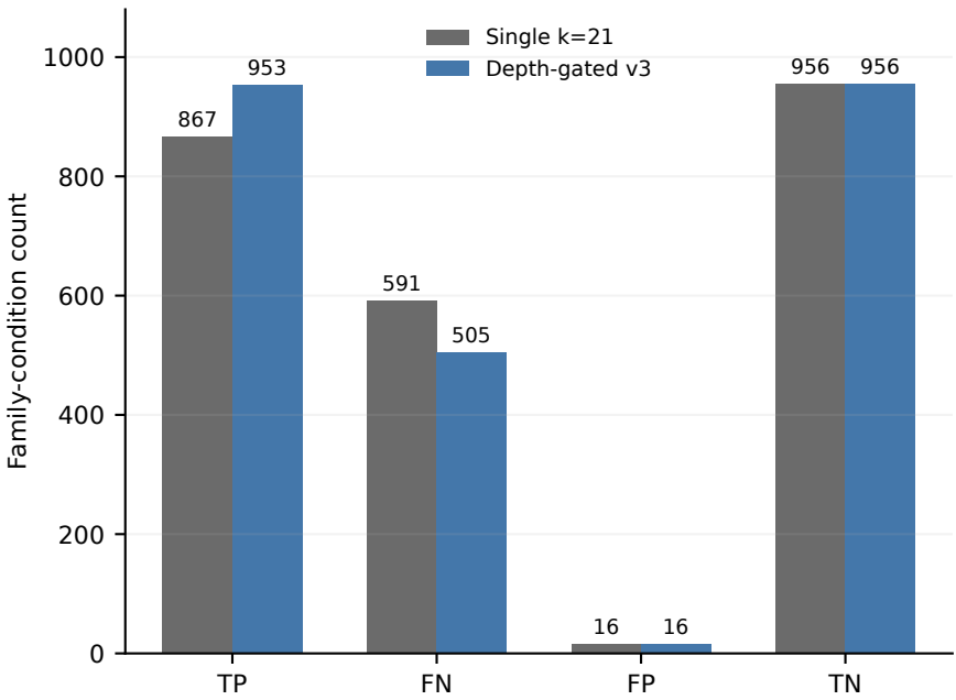
C Held-out confusion counts
