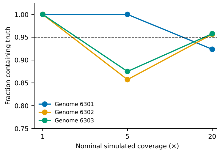
Coverage conditional on availability
