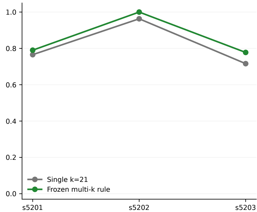
D Sensitivity by fresh genome
