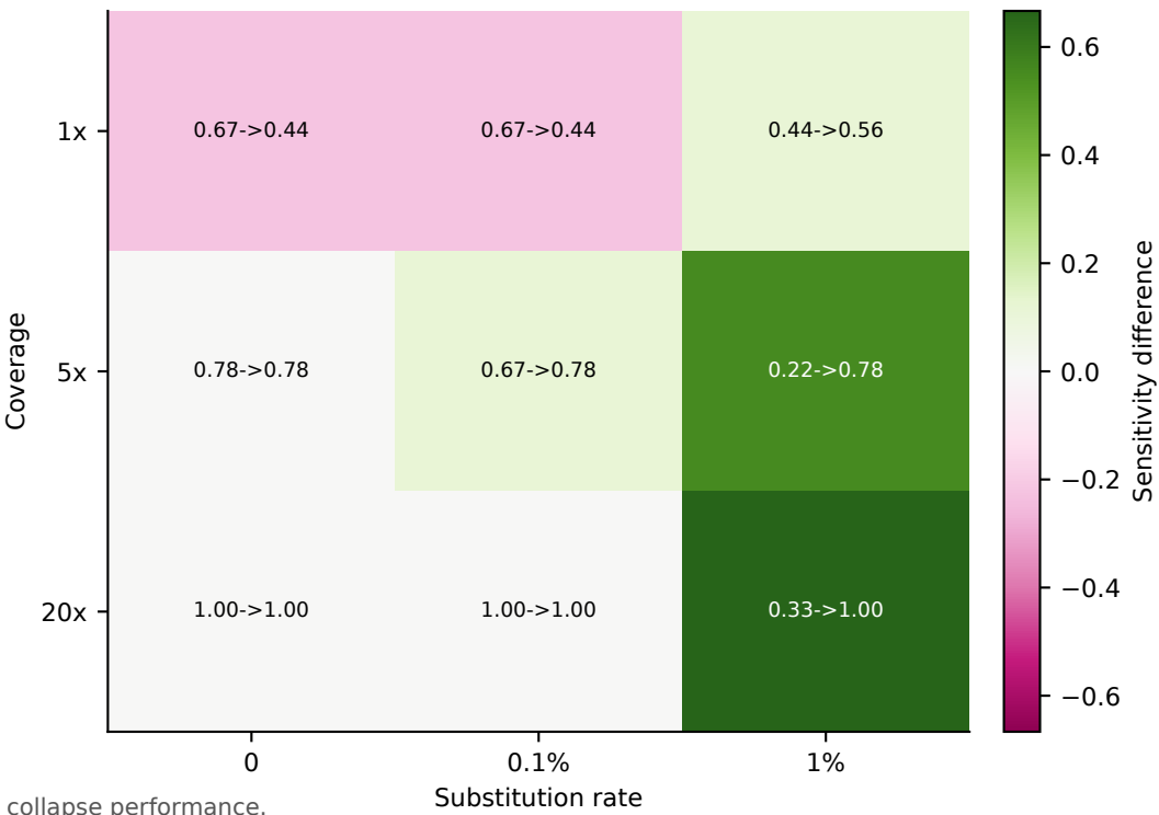
F Recall gain at 50% retention
