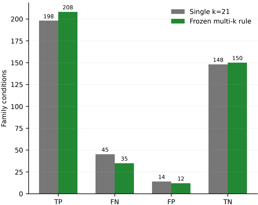
C Confusion counts
