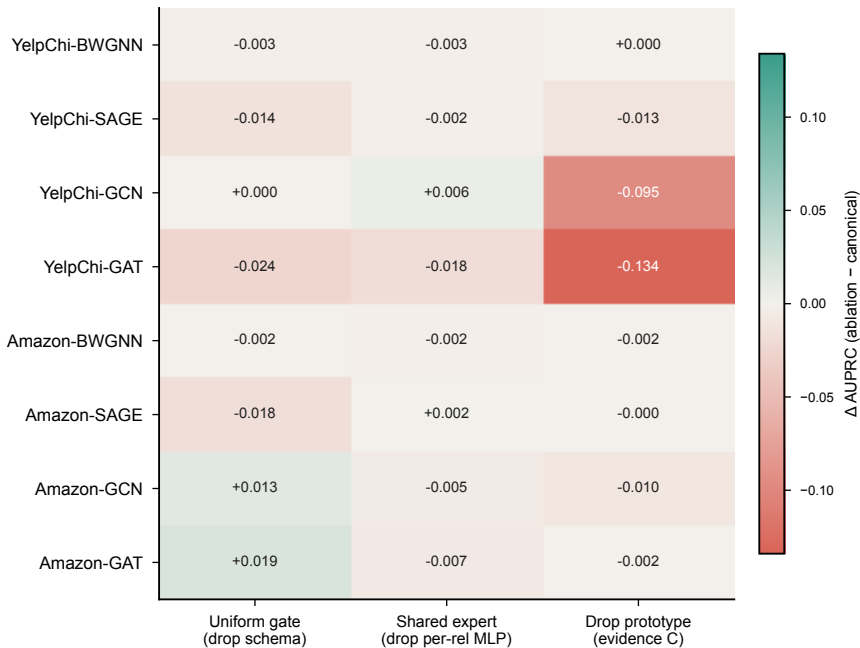
C1 — Law 1: base-strength × evidence-type interaction ( \Delta AUPRC under single-switch ablation)
