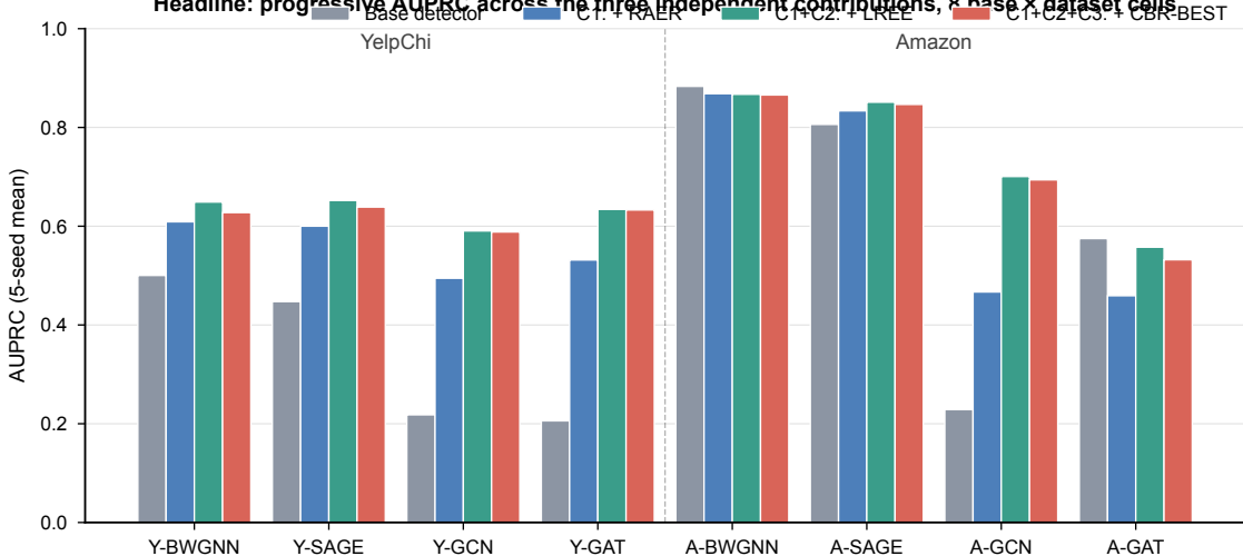
Headline: progressive AUPRC across the three independent contributions, 8 base x dataset cells
