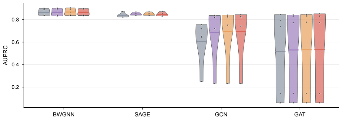
(b) Amazon — 5-seed per-cell distributions across 4 distillation modes
