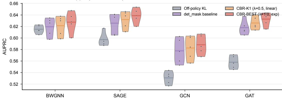
(a) Yelpchi — 5-seed per-cell distributions across 4 distillation modes
