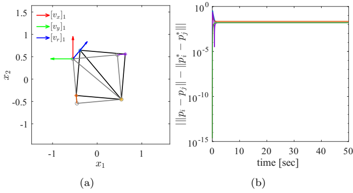
Fig. 4. Shape distortion with an aligned input. (a) An impulse with a component along the local rotational RBM direction excites a rotational motion. (b) The formation deforms, resulting in persistent edge length errors.
