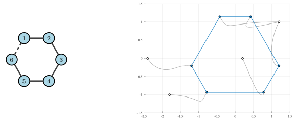
(a) The cycle graph C_6 . (b) Agents converge to a \tau(C_n) -symmetric formation.
