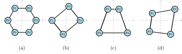
Fig. 1. Symmetric frameworks with C_n as the underlying graph. (a) A C_{6v} -symmetric graph, (b) has a 180^\circ rotation symmetry ( C_2 ), (c) a framework with a reflective symmetry ( C_s ) about the y -axis, and (d) a framework with no nontrivial symmetry.
