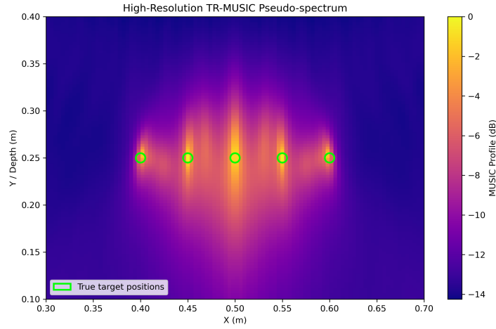
Figure 3: TR-MUSIC pseudo-spectrum using the requested FMC result image, used as a detectability indicator for subwavelength perturbations.
