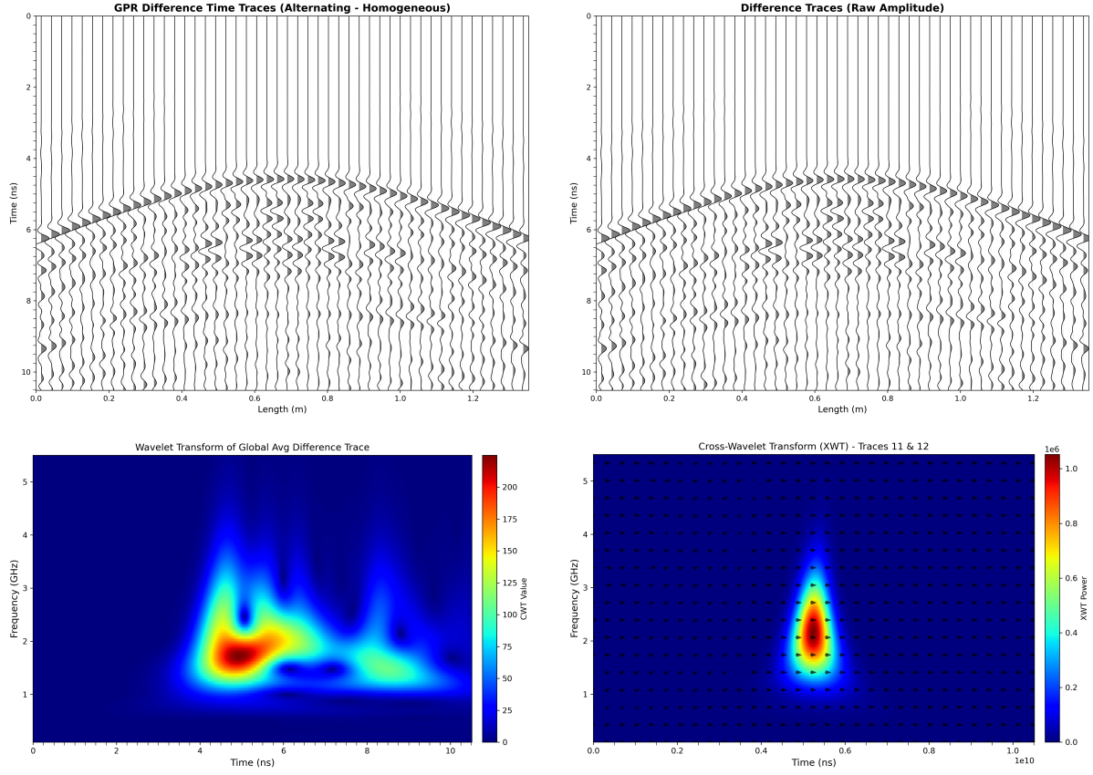
Figure 2: Detection-oriented diagnostics in Diffraction_Experiment : differential response isolation, time-frequency concentration, and inter-trace phase coherence.
