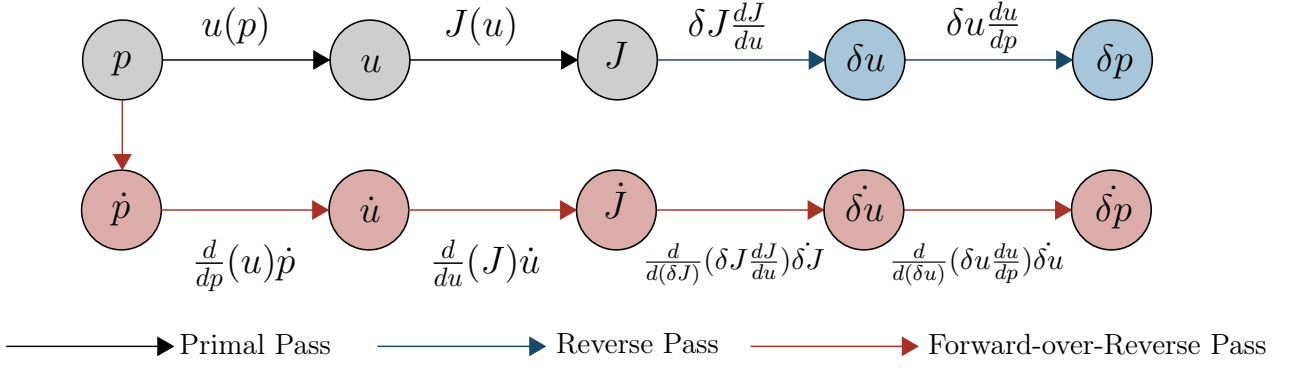
Figure 1. There are far more connections to complete the computational graph - i.e. we need to include arrows from \dot{u} to \delta \dot{u}
