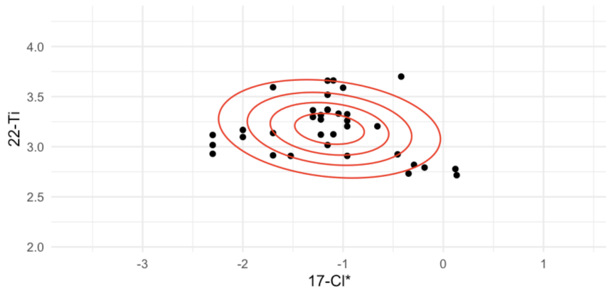
Bivariate Scatterplot of ^{22}\text{Ti} and ^{17}\text{Cl}^* With Two-Dimensional Density Contours
