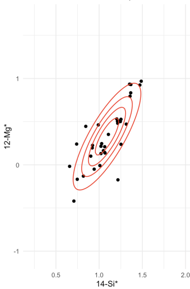
Bivariate Scatterplot of ^{12}\text{Mg}^* and ^{14}\text{Si}^* With Two-Dimensional Density Contours
