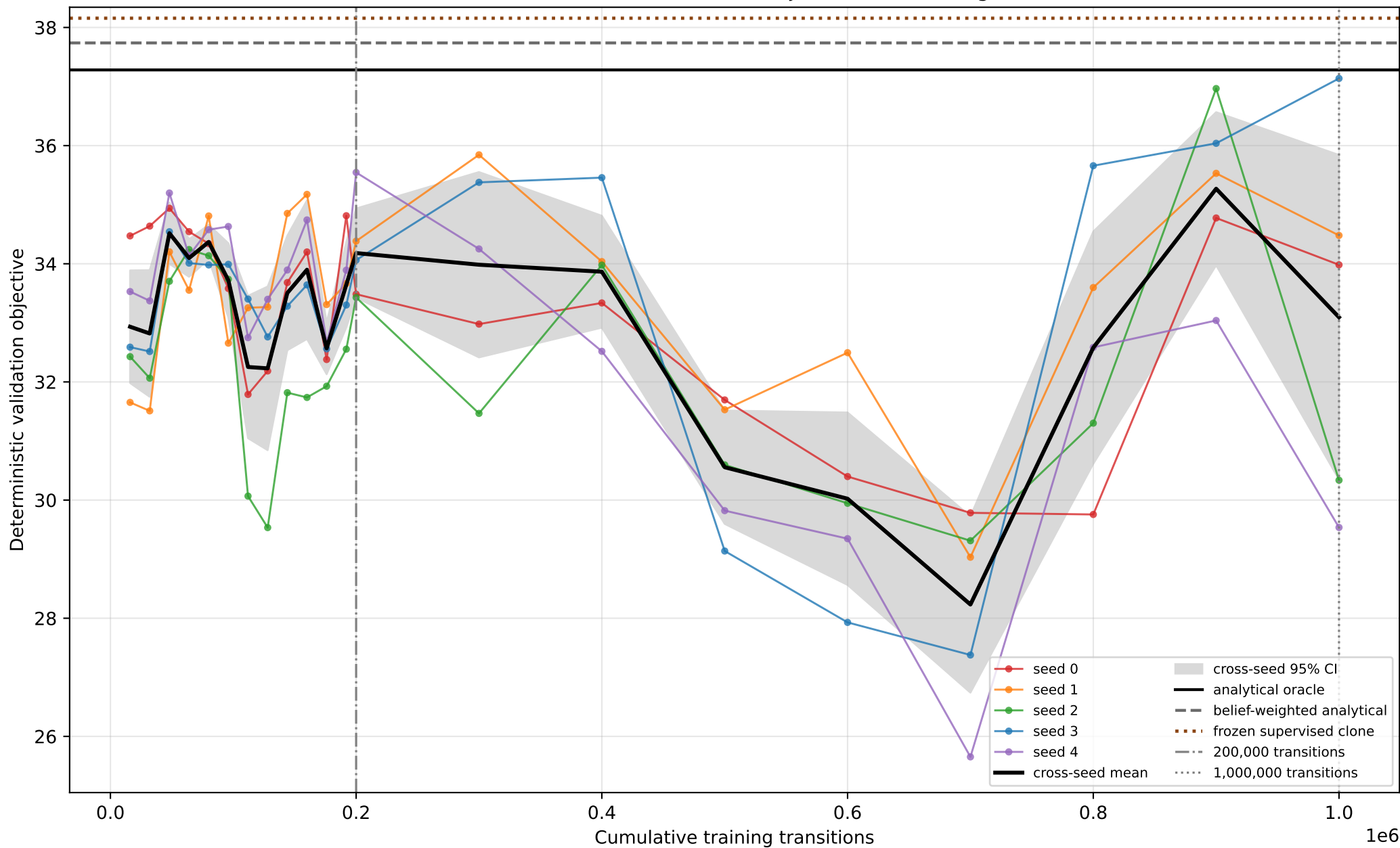
Hamilton belief-state MLP: validation objective vs. training transitions
