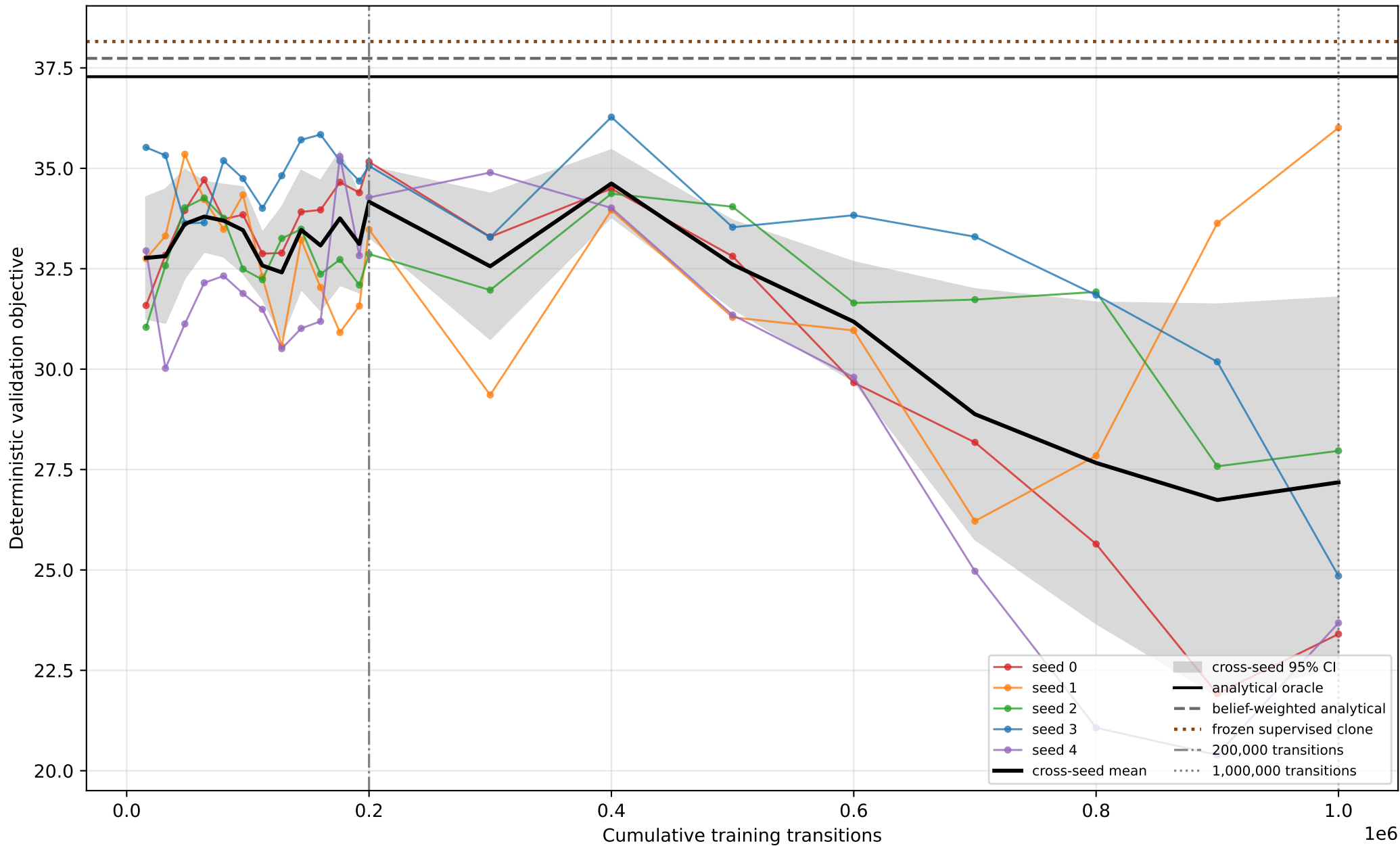
Raw-return LSTM: validation objective vs. training transitions
