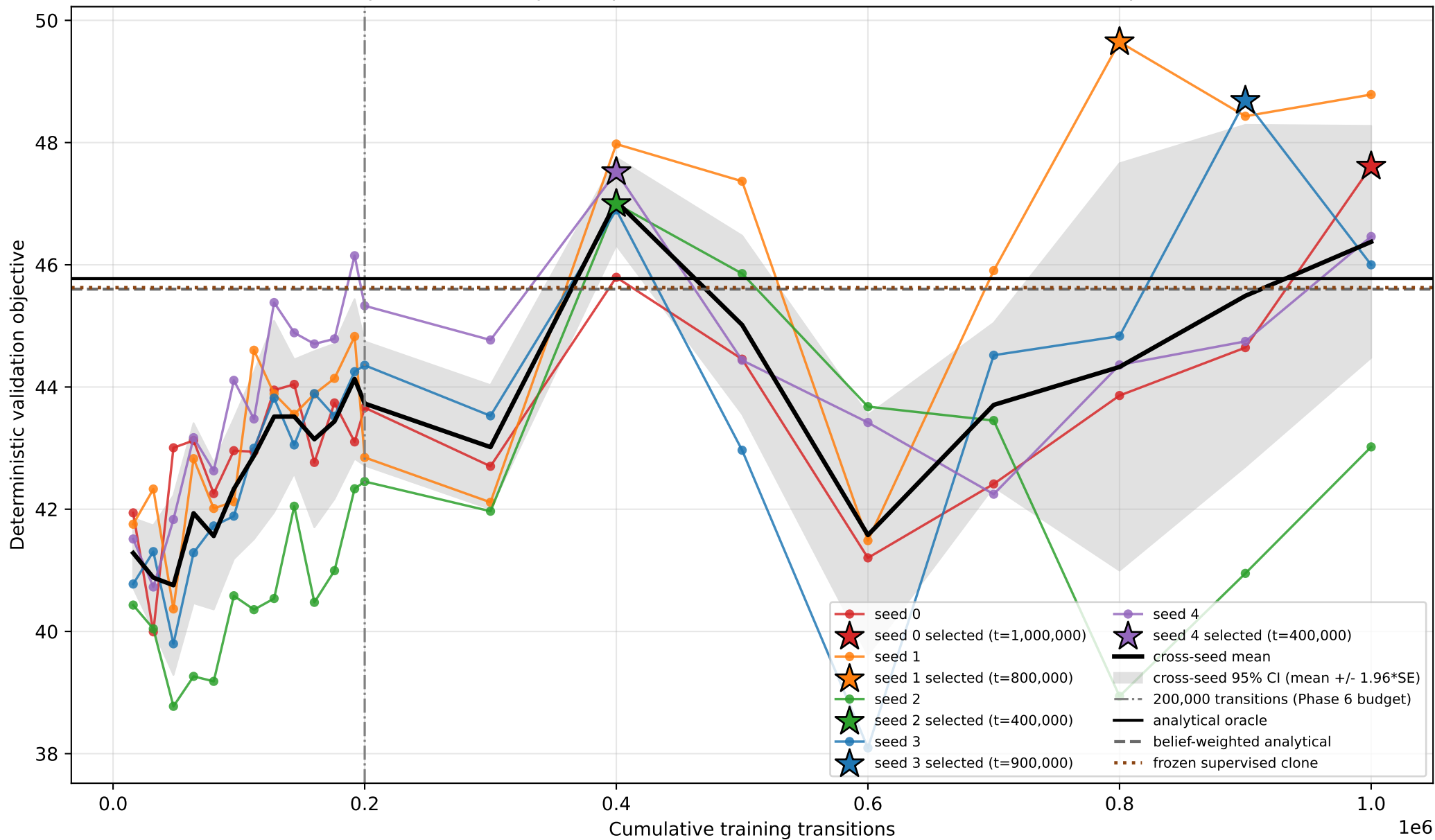
Phase 7 Group B: deterministic validation objective vs. training transitions (raw per-seed checkpoints preserved; stars = each seed's selected checkpoint)
