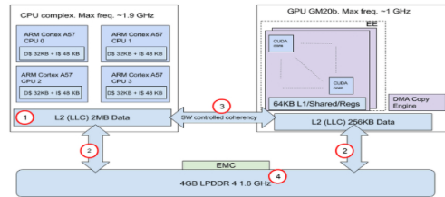
Figure 1: A simplified diagram of the memory hierarchy in the Tegra X1 SoC. Note: The visual representation of the hierarchy is adapted from Burgio et al. (2017, p. 19)
