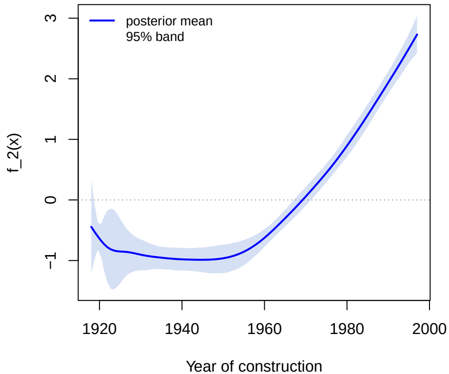
f(yearc) [Model A]
