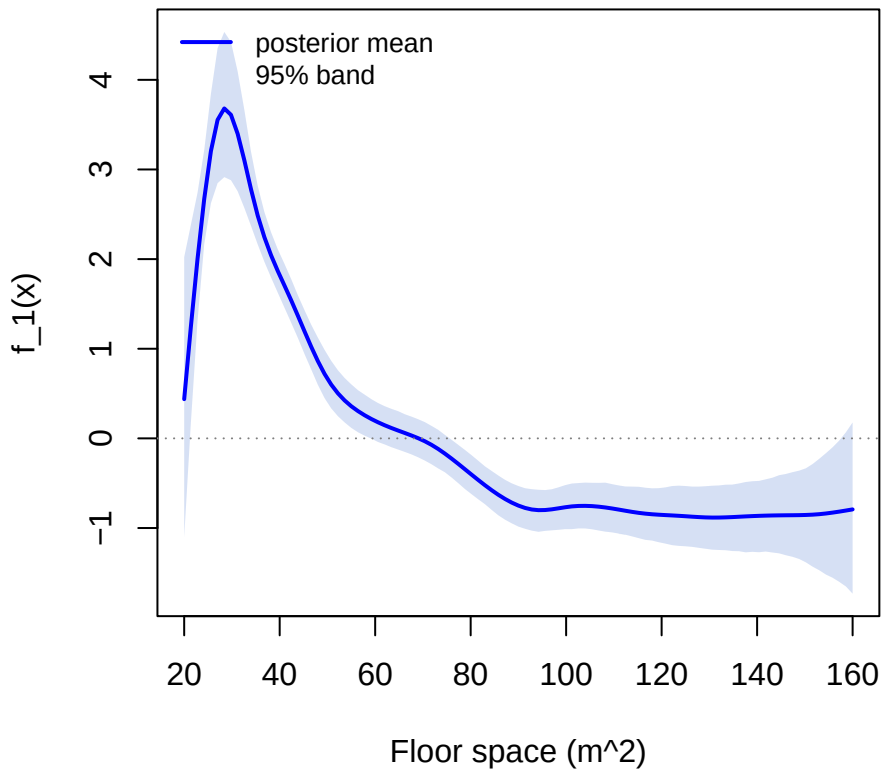
f(area) [Model A]
