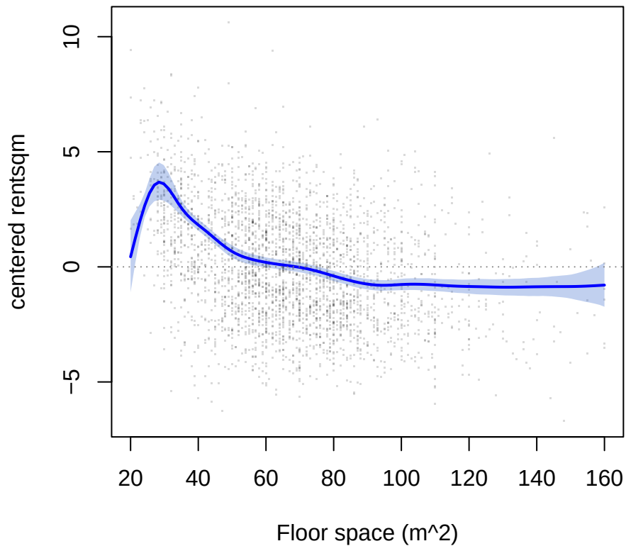
f(area) with data
