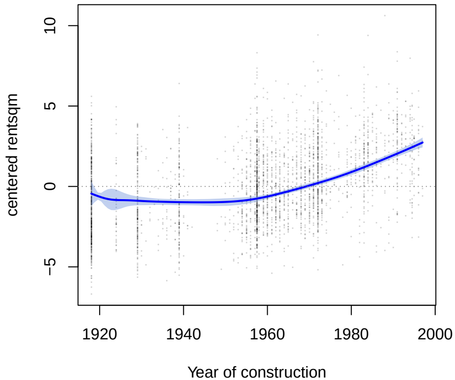
f(yearc) with data
