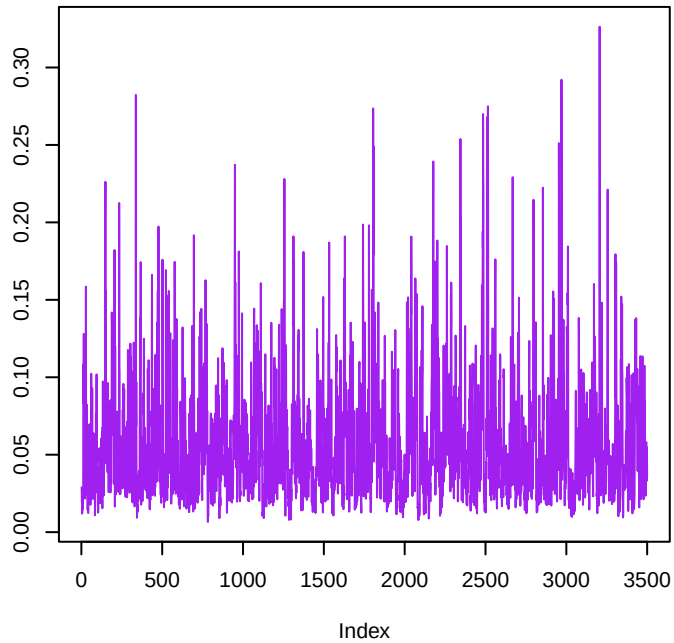
\tau_s^2 (area)
