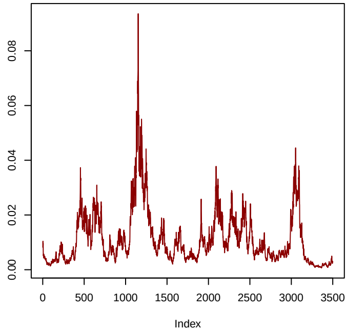
\tau_s^2 (interaction)
