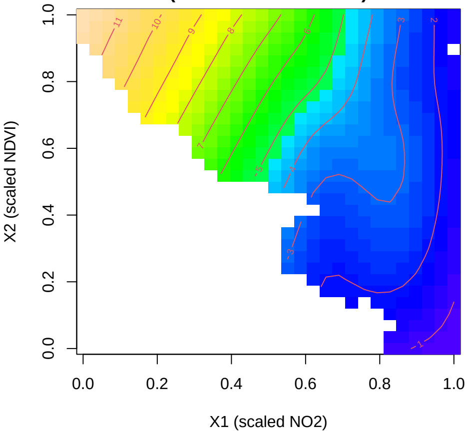
Fitted surface vs (NO 2 , NDVI) (other covs at median)
