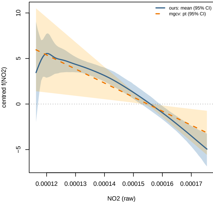
NO2 curve cor: 0.97 | mgcv-in-band: 68%
