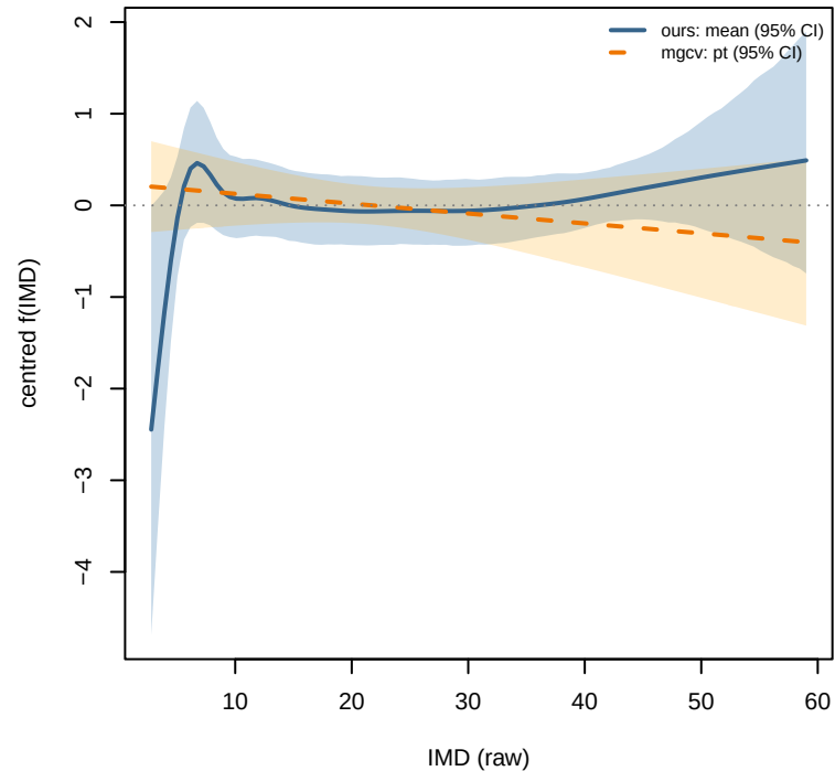
IMD curve cor: -0.51 | mgcv-in-band: 79%
