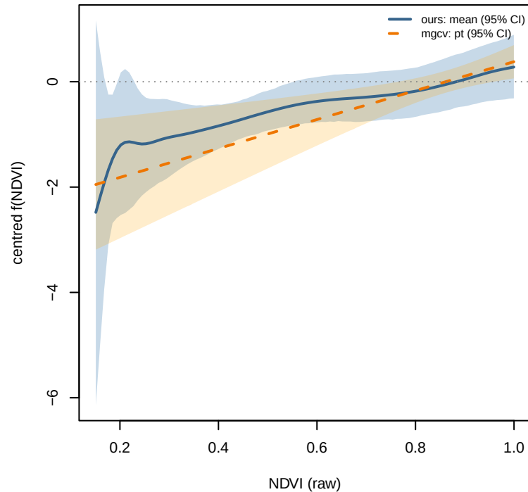
NDVI curve cor: 0.95 | mgcv-in-band: 80%
