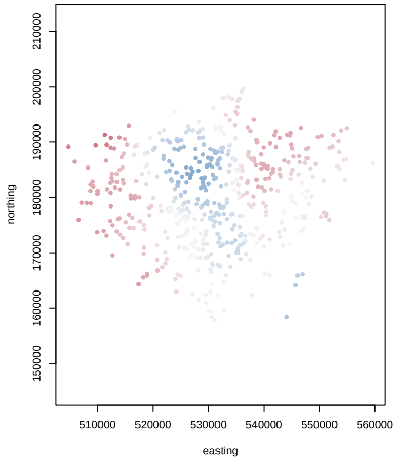
mgcv: s(\text{lon}, \text{lat}) fitted
