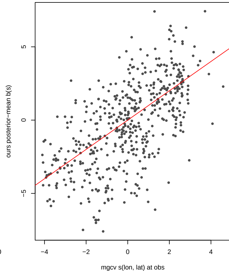
scatter; \text{cor} = 0.618
