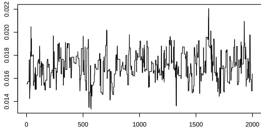
rho (Matern range)
