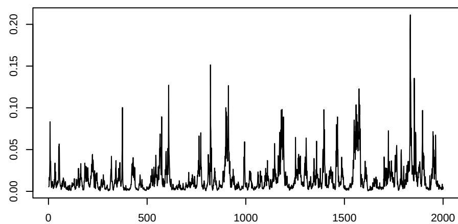
tau2_s[1] (NO2)
