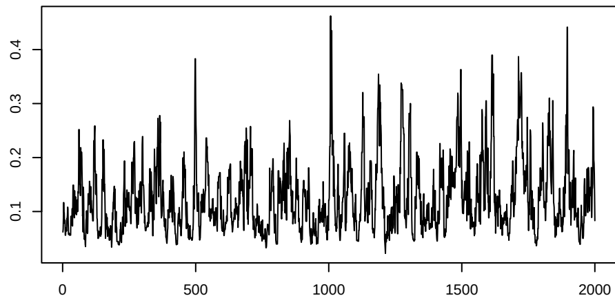
sigma2 (noise)
