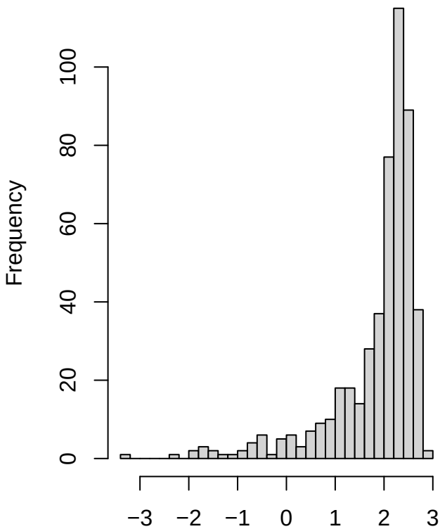
log(y), skew=-2.23
