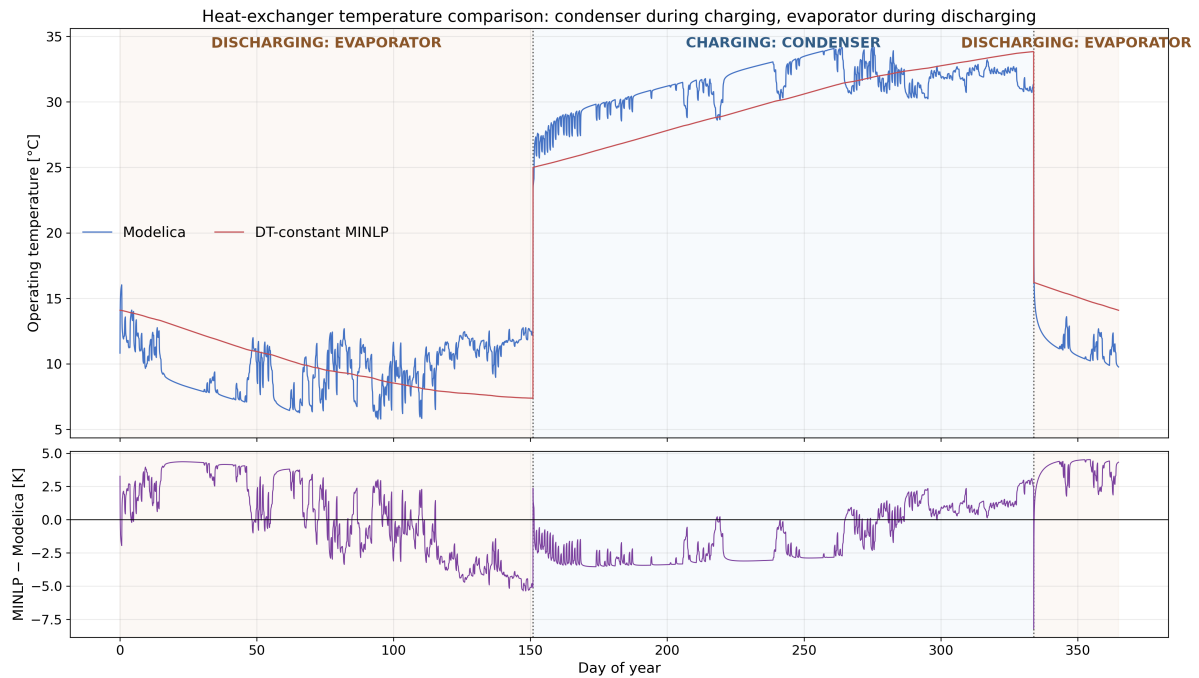
Figure 7: Operating temperatures predicted by the \Delta T -constant MINLP and Modelica. The lower panel shows the paired hourly error, defined as MINLP minus Modelica. Dotted vertical lines indicate the transitions between operating periods.
