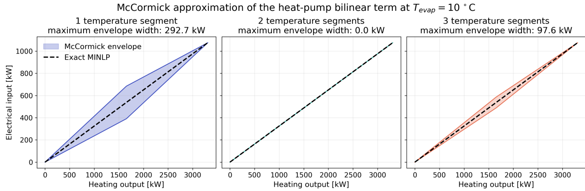
Figure 6: McCormick relaxation using one, two, and three segments for the approximation of the BTES heat-pump bilinear term at T_{\text{evap}} = 10^\circ\text{C}
