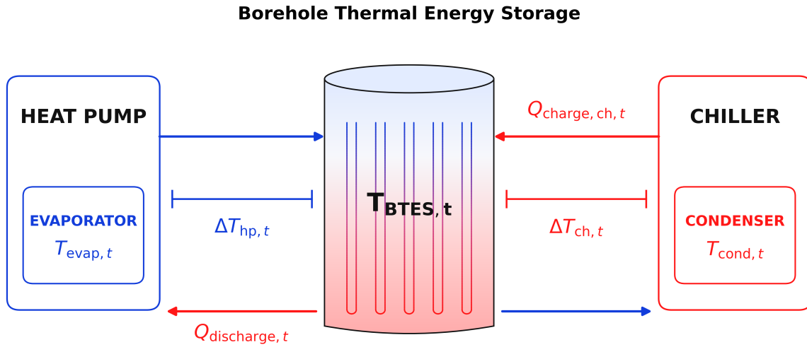
Figure 4: Operating temperatures and temperature differences governing the interaction of the BTES with the heat-pump evaporator during discharge and the chiller condenser during charging. Where T_{BTES} is the average BTES temperature of the system.
