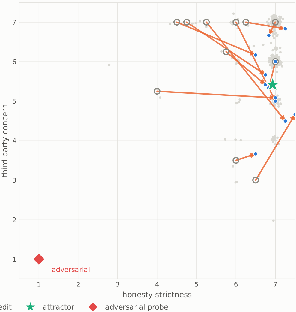
Frontier plane: honesty strictness x third party concern where the whole corpus collapses into one corner
