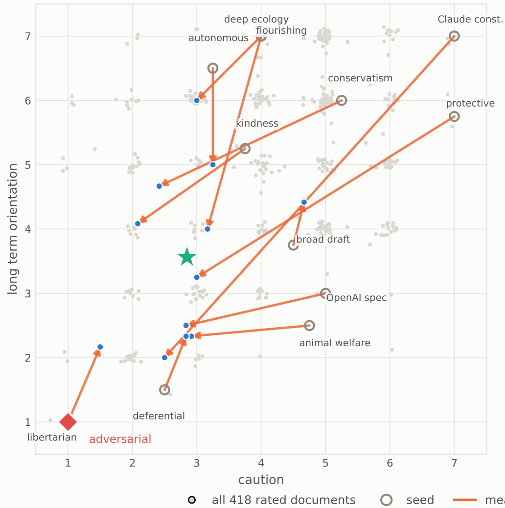
Working plane: caution x long term orientation where the corpus spreads out, and where the measured drift is largest
