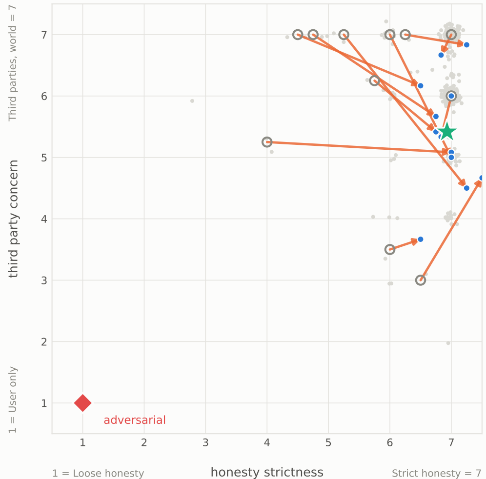
Frontier plane: honesty strictness x third party concern where the whole corpus collapses into one corner
