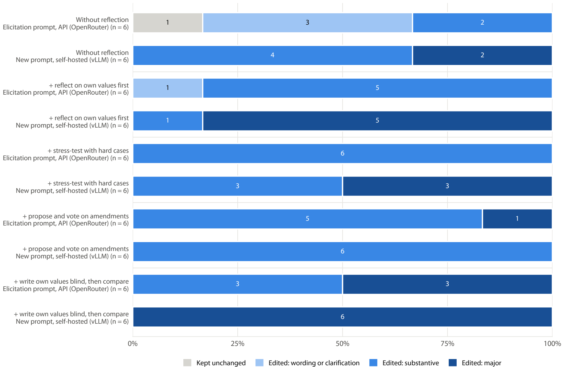
Qwen3.8 27B, broad draft: outcome of each review (edits judged by Claude)
