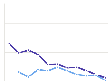
Specificity
