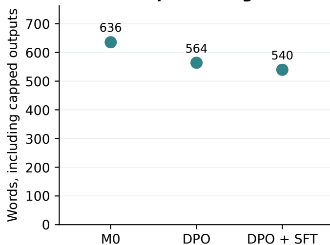
Median response length
