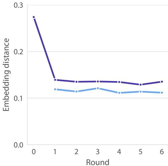
gpt-oss-120b No length limit
