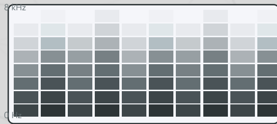
Mel spectrogram
