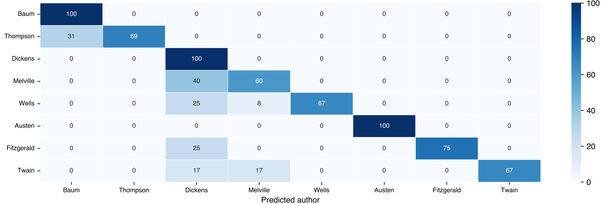
nomic-embed-text-v1.5
