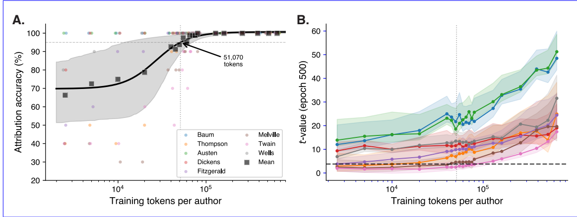
Figure 6: Attribution accuracy vs. corpus size. A. Attribution accuracy as a function of training tokens per author. Small colored dots show per-author accuracy (averaged over 10 seeds); black squares show the mean across all authors for each token count. The black curve is a fitted sigmoid ( R^2 = 0.979 ); the gray ribbon denotes the bootstrap-estimated 95% confidence interval (resampled over authors). The dotted vertical line marks the estimated minimum tokens required to achieve \geq 95\% expected accuracy (51,070 tokens). B. Final-epoch (epoch 500) t -statistics comparing same-author versus other-author cross-entropy losses, plotted as a function of training tokens. Each curve denotes one author; ribbons show bootstrap 95% confidence intervals (resampled over seeds). The dashed horizontal line marks the p < 0.001 significance threshold. The dotted vertical line marks the same token threshold as in Panel A.
