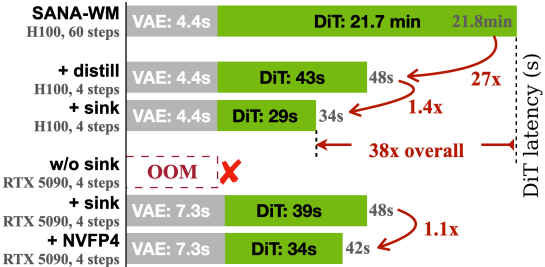
(a). 60s efficiency ablation
