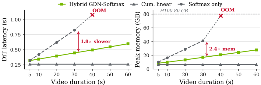
(b). Latency & GPU Memory comparison on H100
