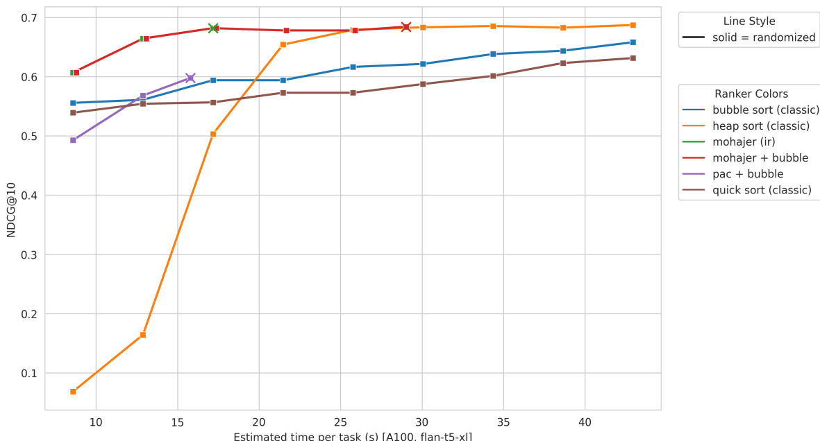
FIGURE 1 TREC DL 2019/2020 (Flan-T5-XL, A100): NDCG@10 vs. avg. time per task (randomized oracle). X marks the point at which a method has completed all its scheduled comparisons (convergence).
