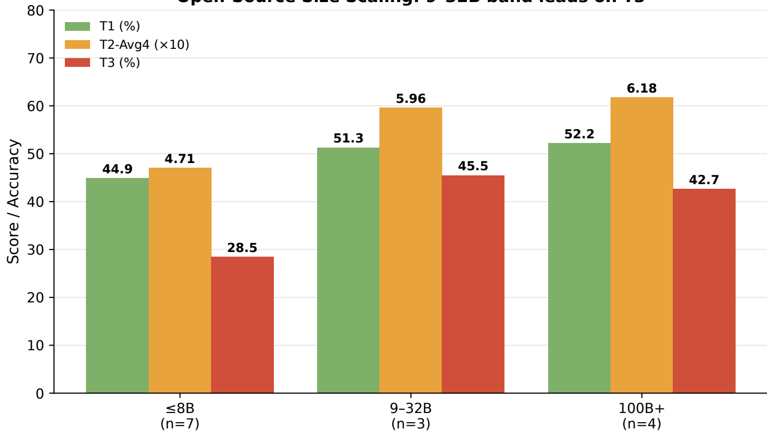
Open-Source Size Scaling: 9-32B band leads on T3
