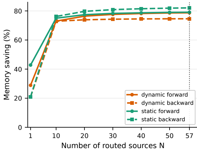
Activation-memory saving
