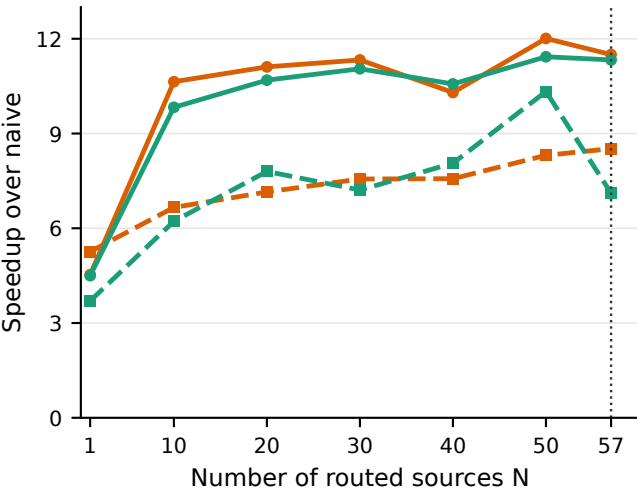
Latency speedup
