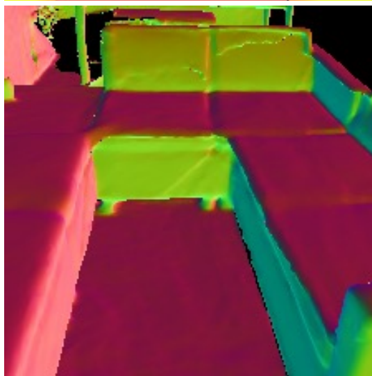
Ground Truth
