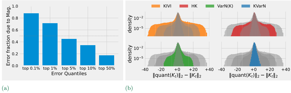
FIGURE 1 (a) What fraction of the top k% largest errors is due to magnitude rather than direction (decomposed as in Eq. 3). Large quantization errors in K are mostly due to incorrect token scaling. To fix outlier errors, the token magnitude needs to be better preserved. (b) Difference of per-token magnitude of quantized K to full-precision K matrix on Qwen3-4B under different 2-bit quantization methods (KIVI [19], HK: Hadamard rotated K , VarN( K ): Variance-Normalized K , and SINQ-KV: our proposed method). Variance normalization prevents the rounding process from scaling the norm of worst-case tokens; the effect synergizes with scale-error reduction by Hadamard rotation. SINQ-KV effectively suppresses magnitude errors, which leads to better end-to-end test-time scaling.
