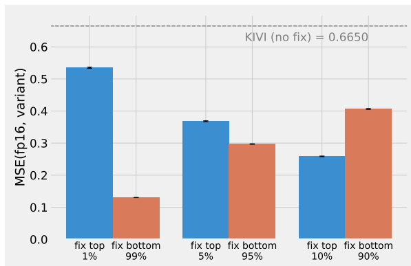
FIGURE 9 Plot to complement Fig. 3. It shows much MSE remains, if we replace the largest top k\% errors with the high precision value. Note that the top 5% of entries contribute less to MSE than the bottom 95%, but their end-to-end KL-divergence impact is greater than that of those bottom 95%.
