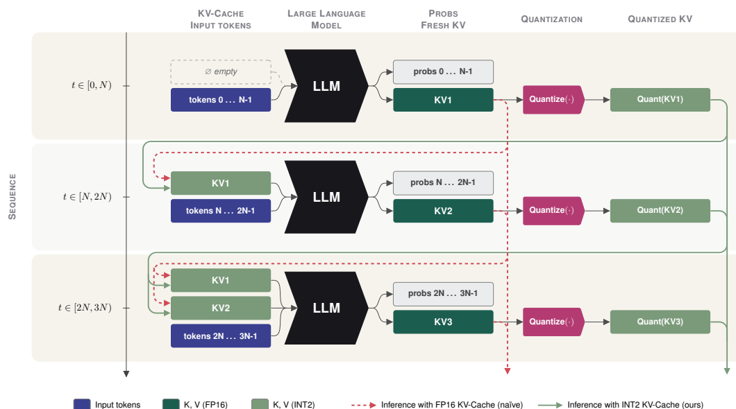
FIGURE 4 Prior KV-Cache quantization papers address the parallel prefill scenario (red dashed arrows). We propose a ‘pseudo-decode’ setting (green solid arrows) to better model decoding errors. We split the sequence into blocks of size b . After every block, the freshly produced K , V are quantized before being written back to the KV-cache. Subsequent blocks access a quantized cache, so quantization error accumulates over time. LLMs operate this way during decoding of long sequences (e.g., in test-time scaling, such as reasoning tasks). SINQ-KV is designed to operate in this regime.
