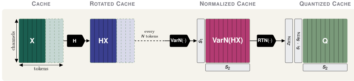
FIGURE 2 Schematic layout of SINQ-KV. Every token is Hadamard-rotated in the channel dimension. After one block of tokens (e.g., 128) of generation, each block is variance-normalized in token and channel dimension, denoted by \text{VarN}(\cdot) . Finally, it is quantized with round-to-nearest (RTN). We store the standard scale and zero-point of the RTN, plus a second scale. At 2.3 average bits per element even with the second scale, SINQ-KV
