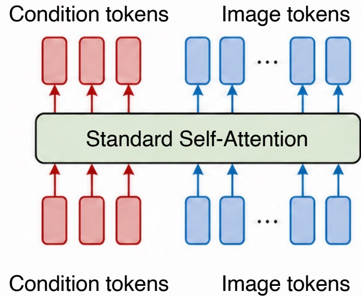
(c) In-Context Concatenation
