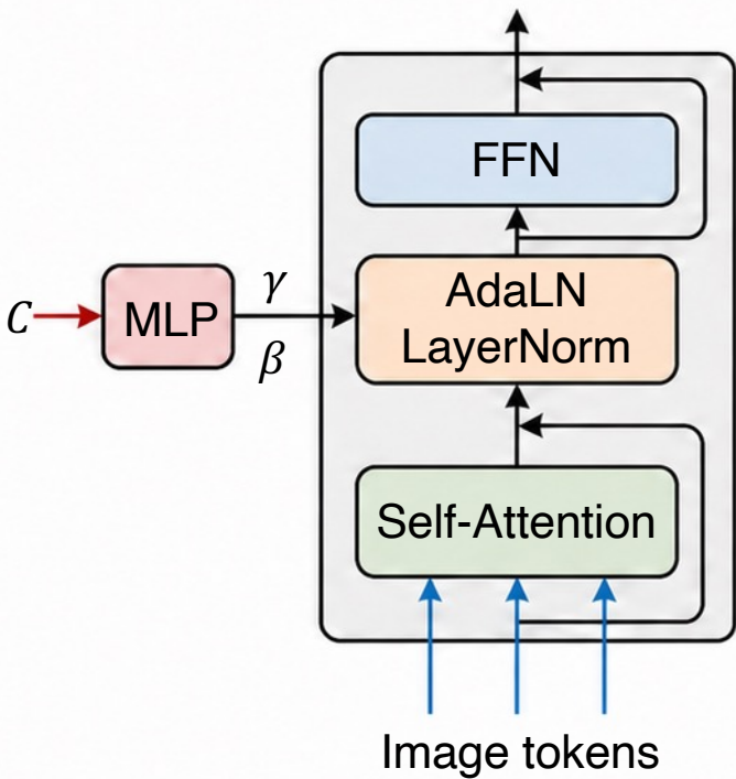
(a) AdaLN Modulation
