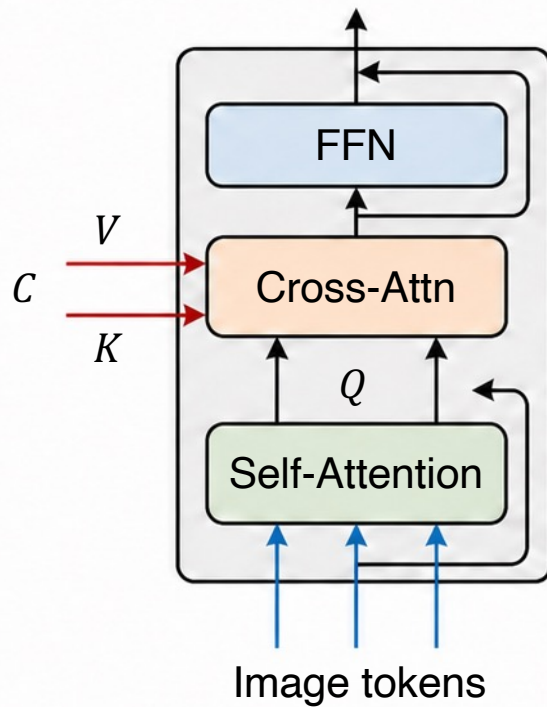
(b) Cross-Attention
