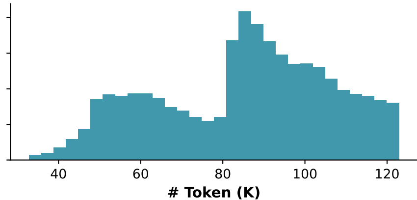
OCR-needle
