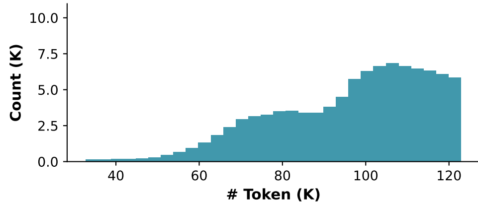
OCR-full
