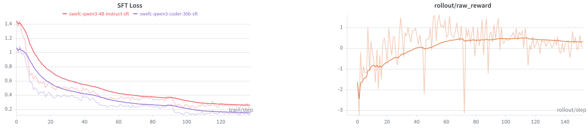
Figure 6: Training curves for the reported FastContext models. Left: supervised fine-tuning loss during policy initialization. Right: reinforcement-learning reward during task-grounded policy refinement.
