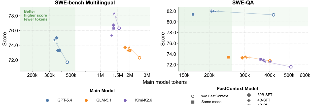
Figure 1: SWE-bench Multilingual and SWE-QA score versus main-model token usage, where FastContext shifts coding agents toward a better score–token tradeoff: cost less and archive more.
