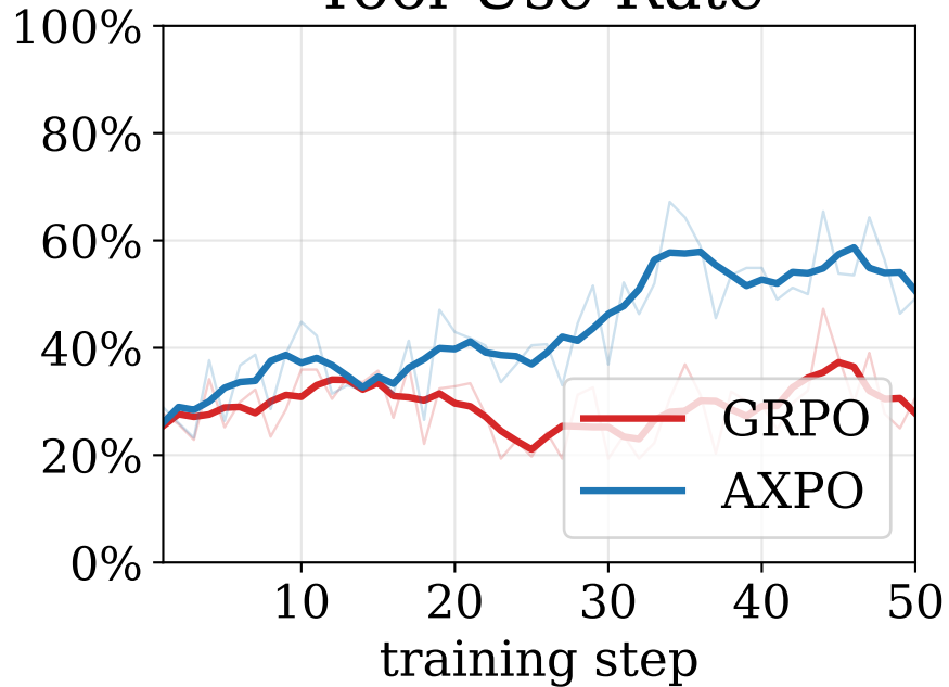
Tool-Use Rate
