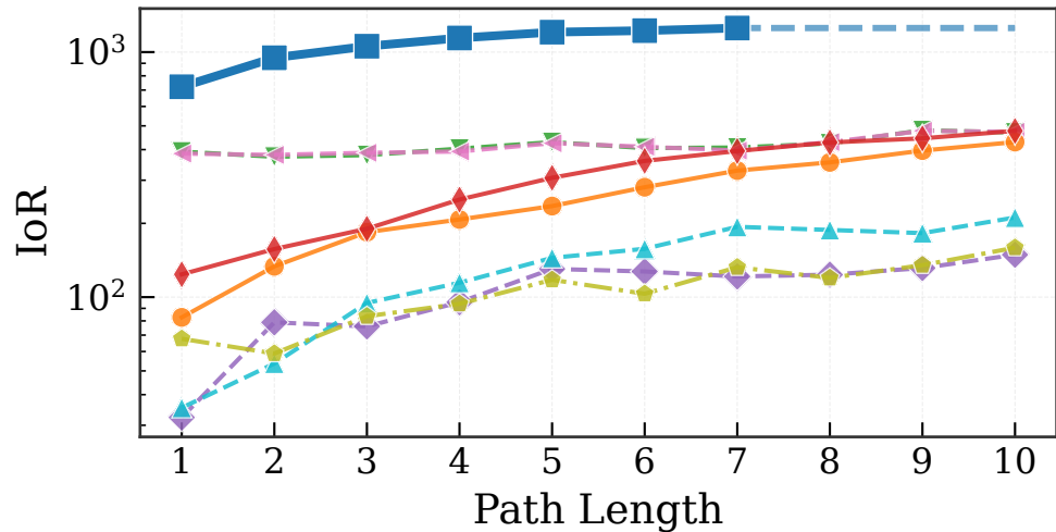
Amazon-Book — IoR
