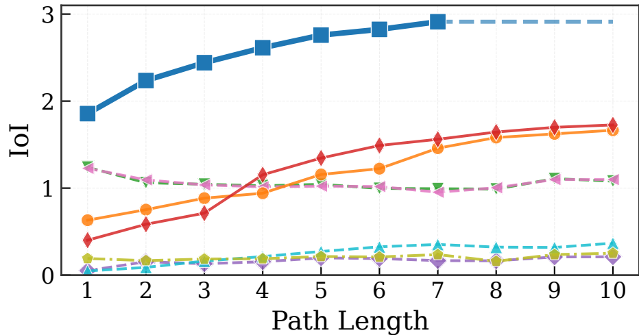
Amazon-Book — IoI
