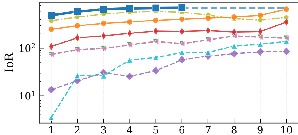
MovieLens-1M — IoR
