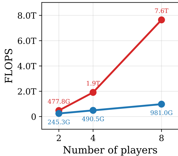
Self-attention FLOPS (analytical)
