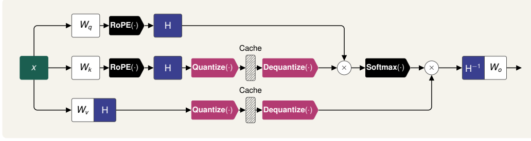
Figure 7: Arrangement of Hadamard transforms in an attention layer in our method.
