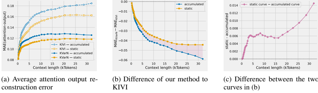
Figure 5: Average reconstruction error after quantization across all attention layer outputs in Qwen3-4B. (a) Our method has smaller error than KIVI at all context lengths. As discussed in Sec. 3.2 errors accumulate over time. Prior work considers the static case (orange) here we consider the dynamic accumulation (blue) (b), (c) KVarN has an increasing advantage over KIVI as contexts get longer.
