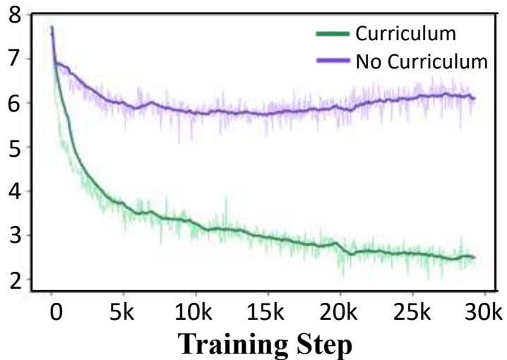
Accept Length
