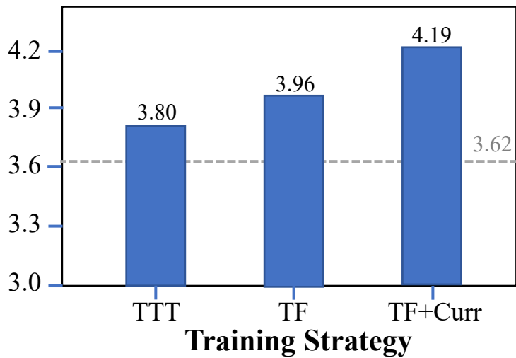
Accept Length
