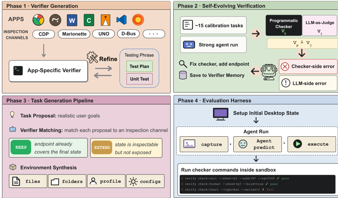
FIGURE 1 Overview of the OpenComputer verifiable software-world synthesis pipeline. Phase 1 generates app-specific verifier endpoints over the most reliable inspection channels and validates it with unit and integration tests for structured, machine-checkable state. Phase 2 closes a self-evolving loop: calibration tasks drive a strong agent run, an LLM evaluator and the programmatic verifier produce verdicts that disagreement analysis attributes, and verifier memory – checker/endpoint/doc fixes refine the verifier with execution-grounded feedback. Phase 3 proposes user goals, filters by complexity and data generatability, matches against the verifier, synthesizes the environment, and emits a final task instance. Phase 4 runs the agent and computes the reward.
