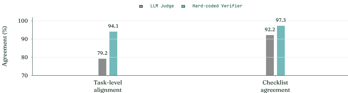
FIGURE 3 Alignment with human adjudication on a 120-task comparison set.
